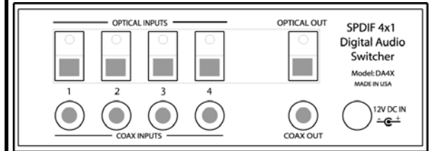
Figure 1 -Connectors
