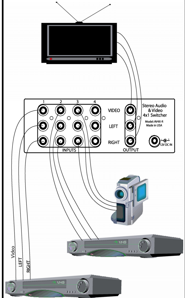
Figure 2 - Typical Setup
